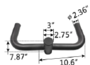
Double Side Bullhorn ZL-RB2.5D180H-D
