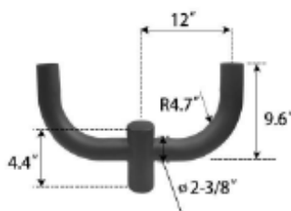
180° Double Bullhorn ZL-RB2.5D180-D
