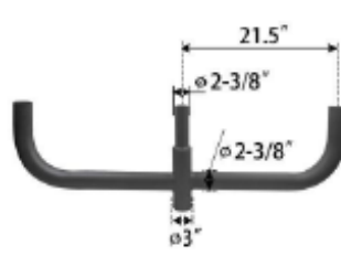
180° Triple Bullhorn ZL-RB2.5TR180-D
